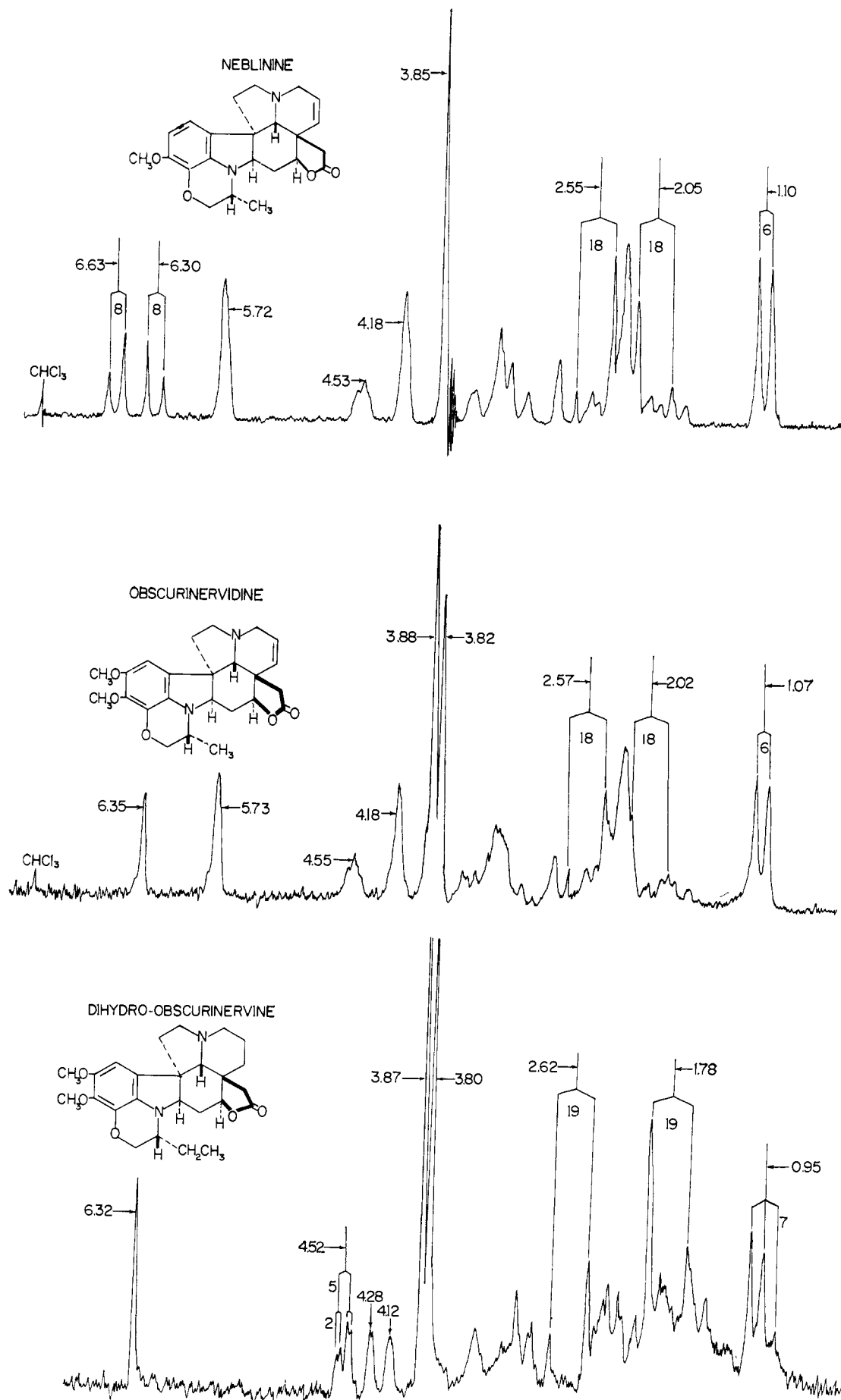
Fig. 2.—N.m.r. spectra of neblinine (IIe), obscurinervidine (II d ), and dihydroobscurinervine (IIa).
